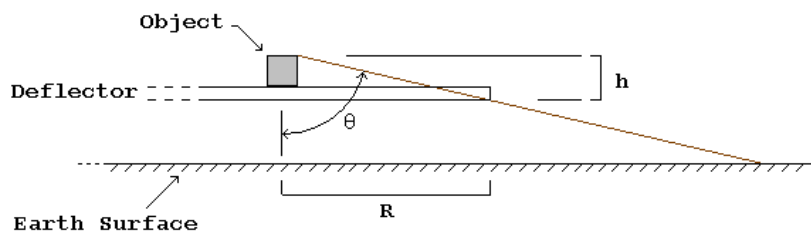
Figure 11 – Size Requirements for a Disk Shaped Deflector
