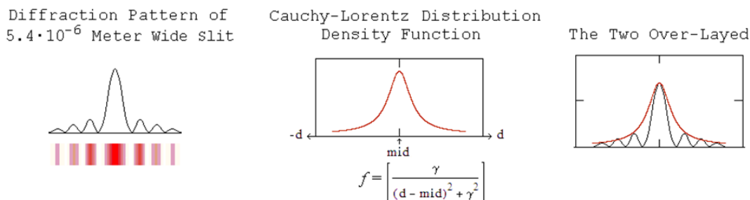
Figure 16 - The Cauchy-Lorentz Distribution Diffraction Pattern Envelope
