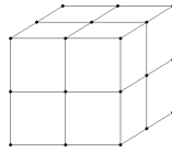
Figure 6 - A Small Piece of a Cubic Crystal
